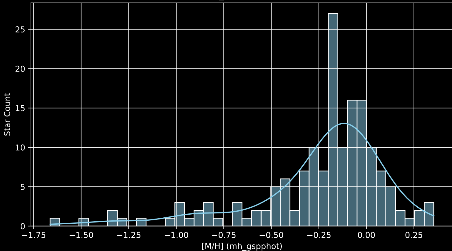
APOGEE DR17 Field: [225+04 [M/H] (mh_gspphot) (n= 161)
