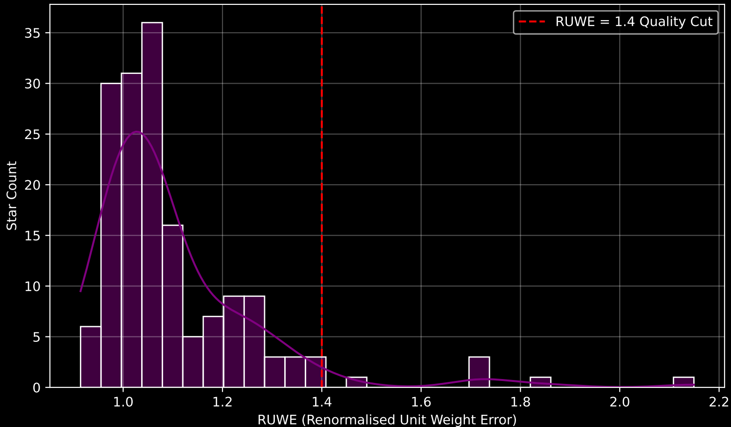
GAPOGEE DR17 Field [225+04] RUWE Distribution (n= 164)
