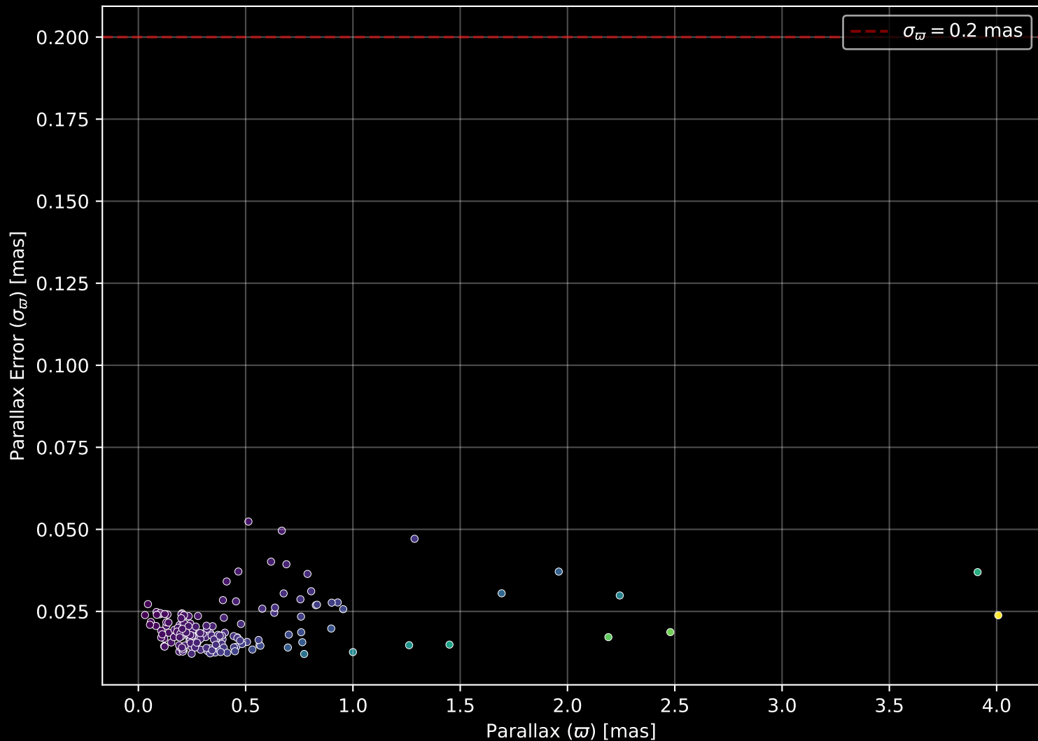
APOGEE DR17 Field: [225+04] Parallax Quality (n= 164)
