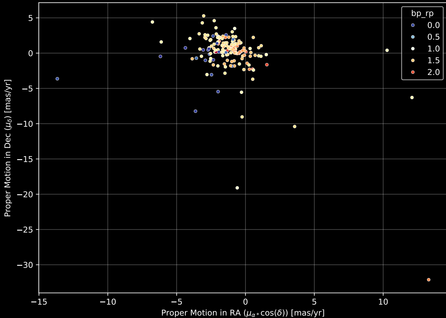
APOGEE DR17 Field: [225+04] Proper Motion Diagram (n= 164)
